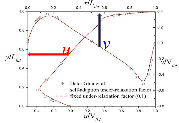
Re=1000 in 40 × 40 grid
