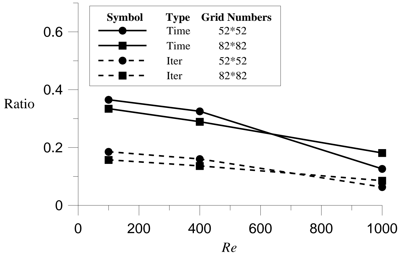
Ratios of CPU time and iteration numbers
