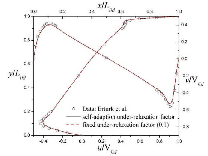
Re=2500 in 80 × 80 grid
