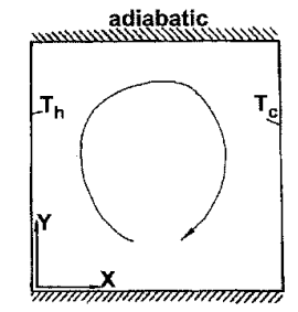
(3) natural convection in a square cavity
