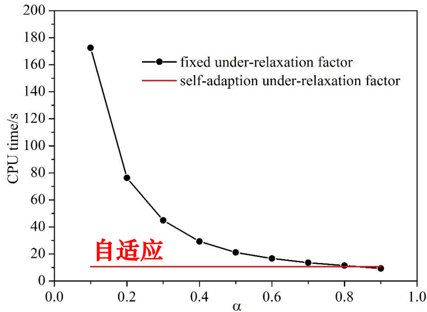
Re=1000 in 40 × 40 grid
