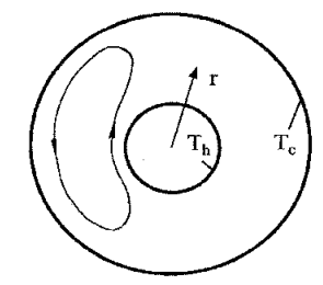
(4) natural convection in a horizontal annular
