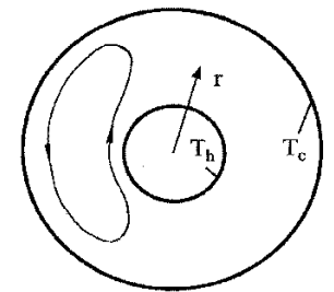
(4) natural convection in a horizontal annular
